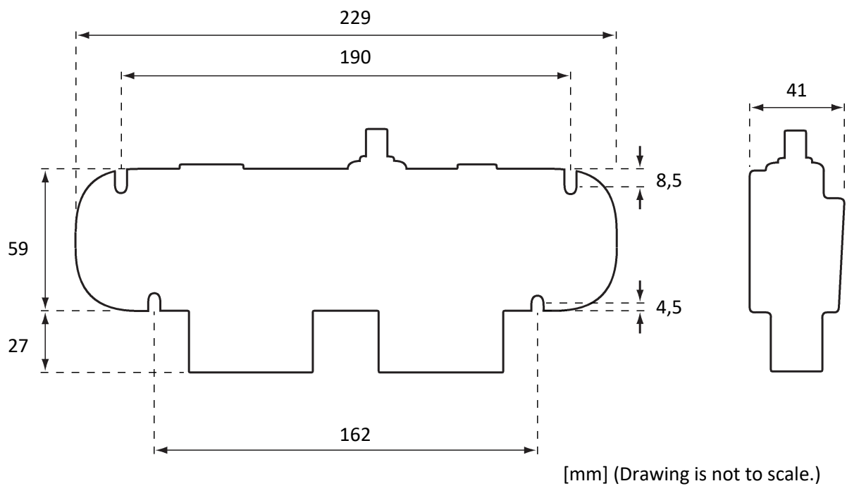
Figure 5.1: Dimensions
